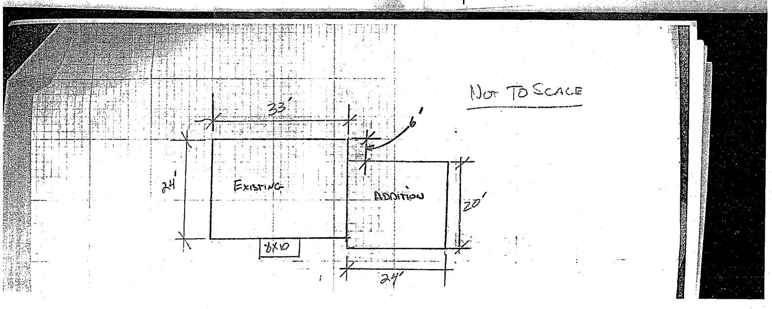
Floorplan
